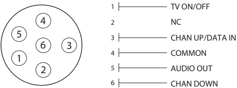
Pillow Speaker Interface Pinout
